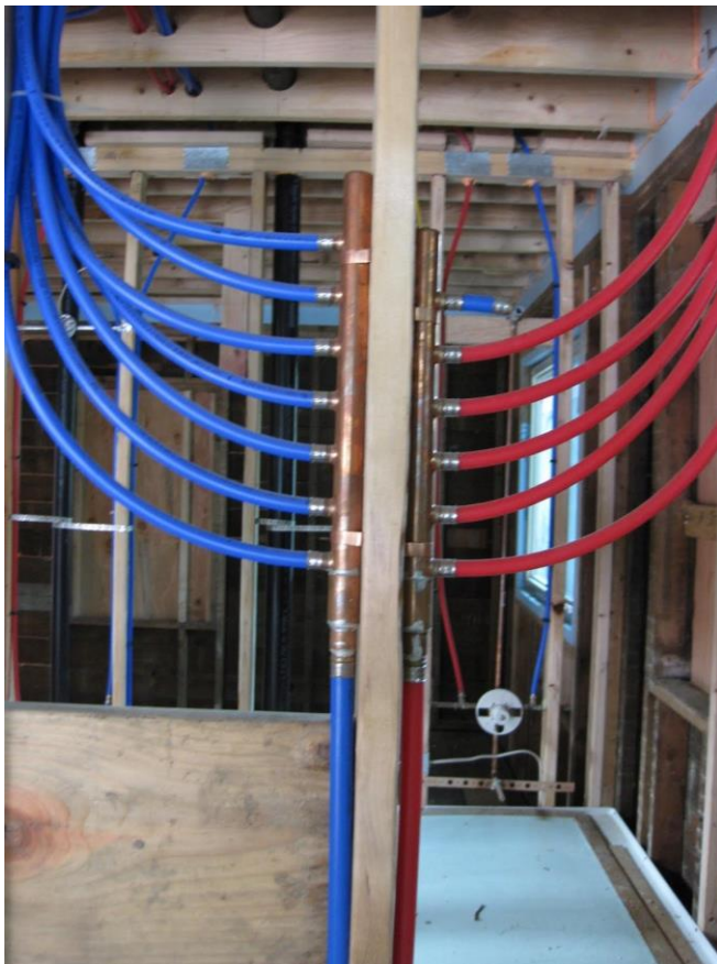
Typical Potable water distribution
