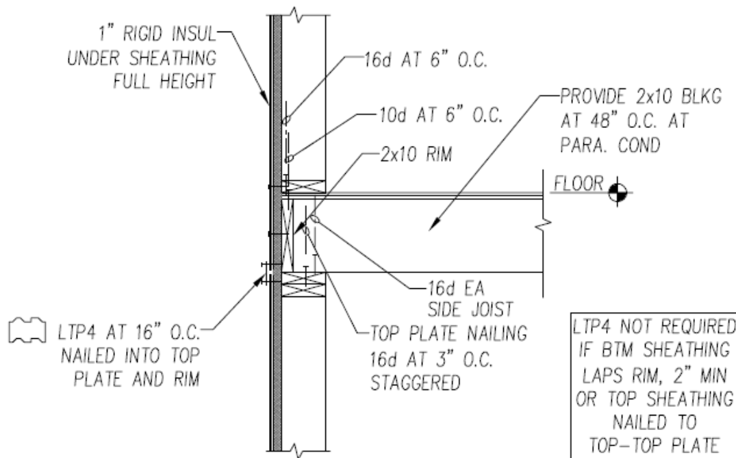
Plan detail showing closed cell foam sheets under cdx plywood on exterior wall
